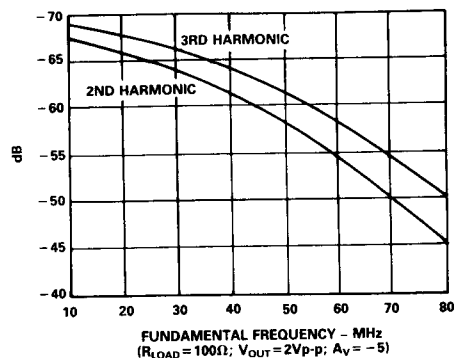
Harmonics vs. Frequency
