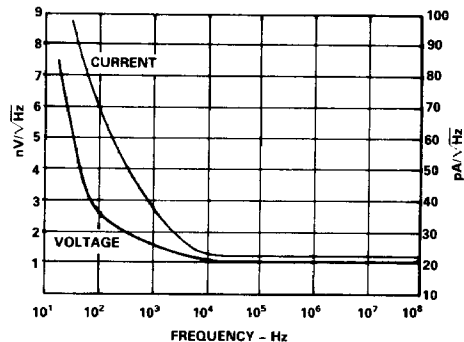
Noise vs. Frequency
