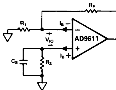
Figure 7. Reducing Offset Drift
