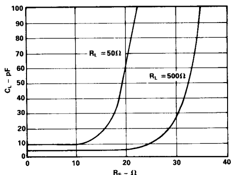
Figure 5. Output Capacitance vs. Compensation
