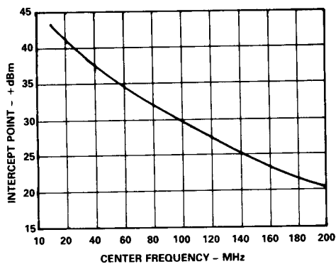
3rd Order Two-Tone Intermod Intercept (Gain = -5; R_{LOAD} = 50\Omega )
