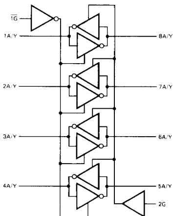
Am54S/74S242
