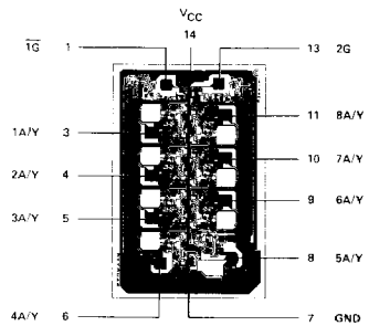
Am54S/74S243
