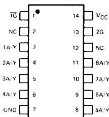
Am54S/74S243
