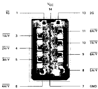
Am54S/74S242
