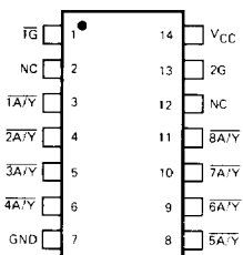
Am54S/74S242
