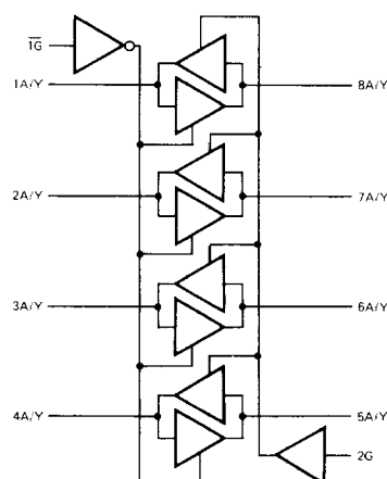
Am54S/74S243
