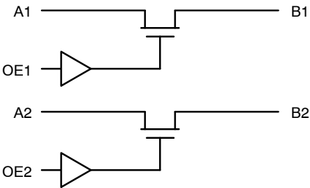
Figure 4. Logic Diagram
