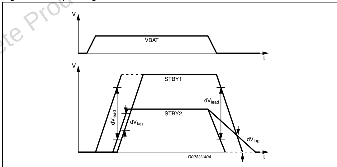
Figure 6. Sequencing function
