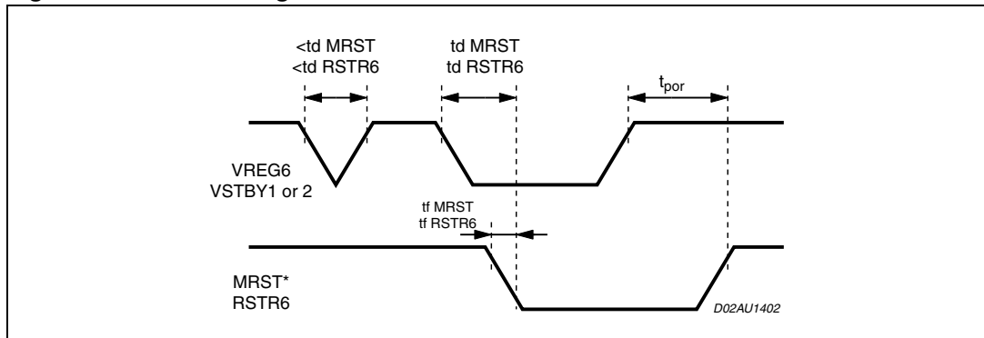
Figure 5. SLEW function
