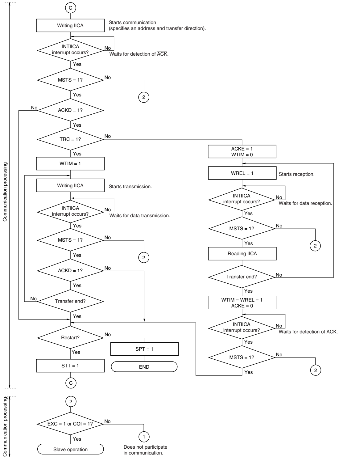
Figure 14-29. Master Operation in Multi-Master System (3/3)
