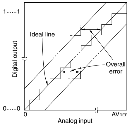
Figure 12-17. Overall Error
