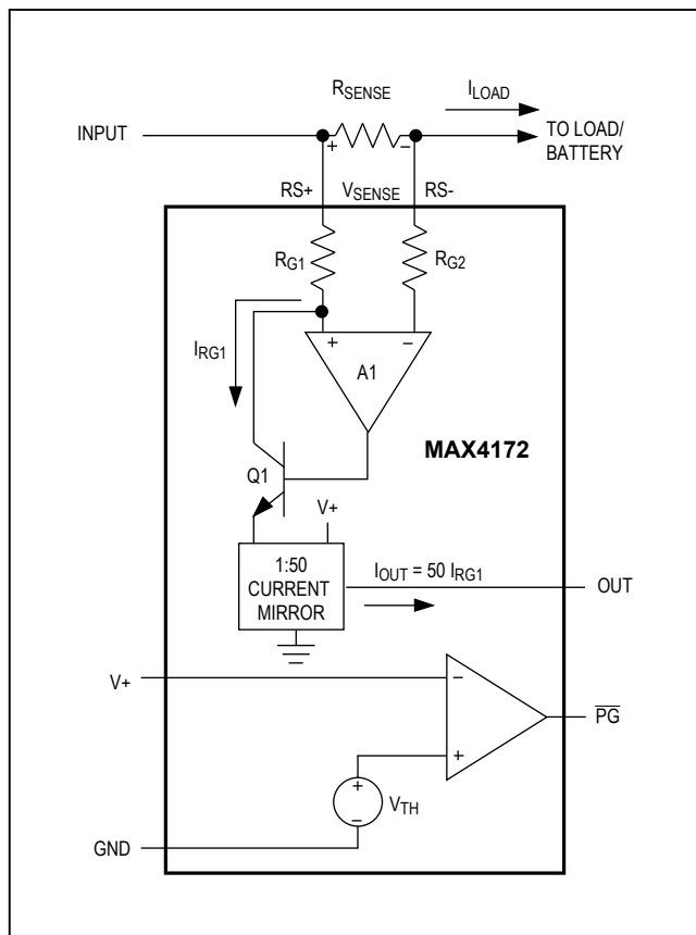
Figure 1. Functional Diagram
