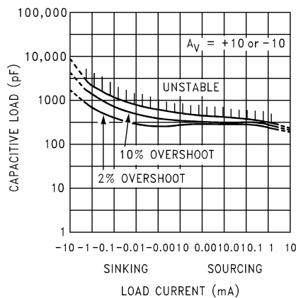
Stability vs Capacitive Load
