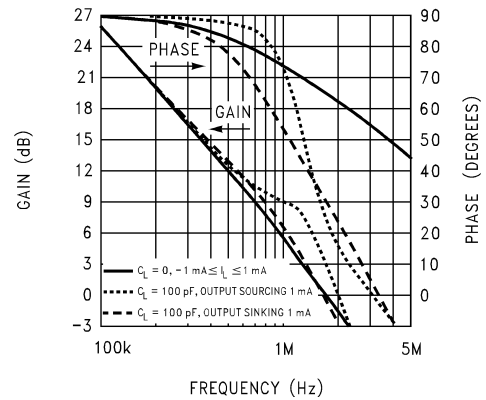
Frequency Response vs Capacitive Load
