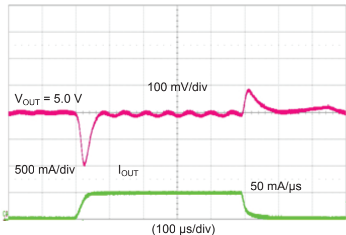
Transient Response 0 to 0.5 A Load Step at V_{IN} = 12 \text{ V} for 5 V_{OUT} , 2 MHz design example
