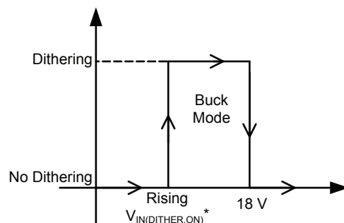
Figure 3: V_{IN} Rising Dithering Threshold
