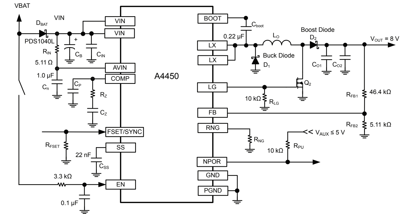
Figure 17: Schematics of 8 V OUT Design Example at 2 MHz
