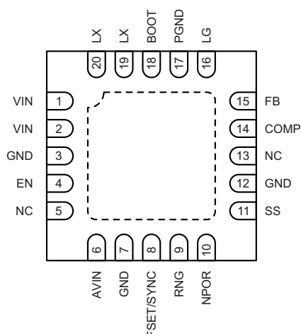
Package ES, 20-Pin QFN Pinout Diagram
