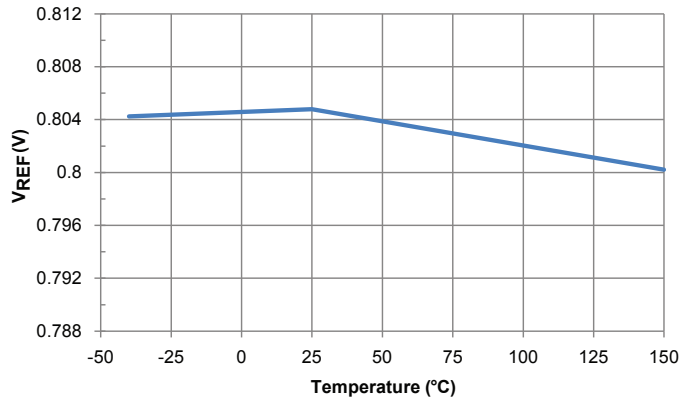
Reference Voltage versus Temperature
