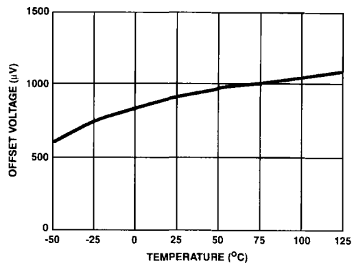
FIGURE 10. OFFSET VOLTAGE vs TEMPERATURE
