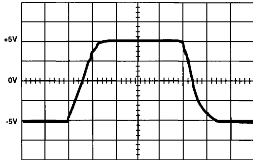
FIGURE 3. HA-5111 LARGE SIGNAL TRANSIENT RESPONSE
