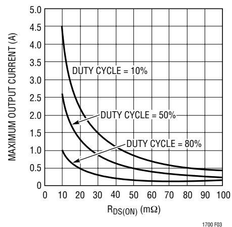
Figure 3. Maximum Current vs R_{DS(ON)}
