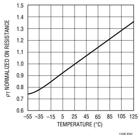
Figure 2. R_{DS(ON)} vs Temperature
