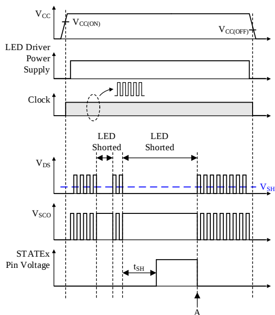
Figure 11-3. Waveforms during Short Detection
