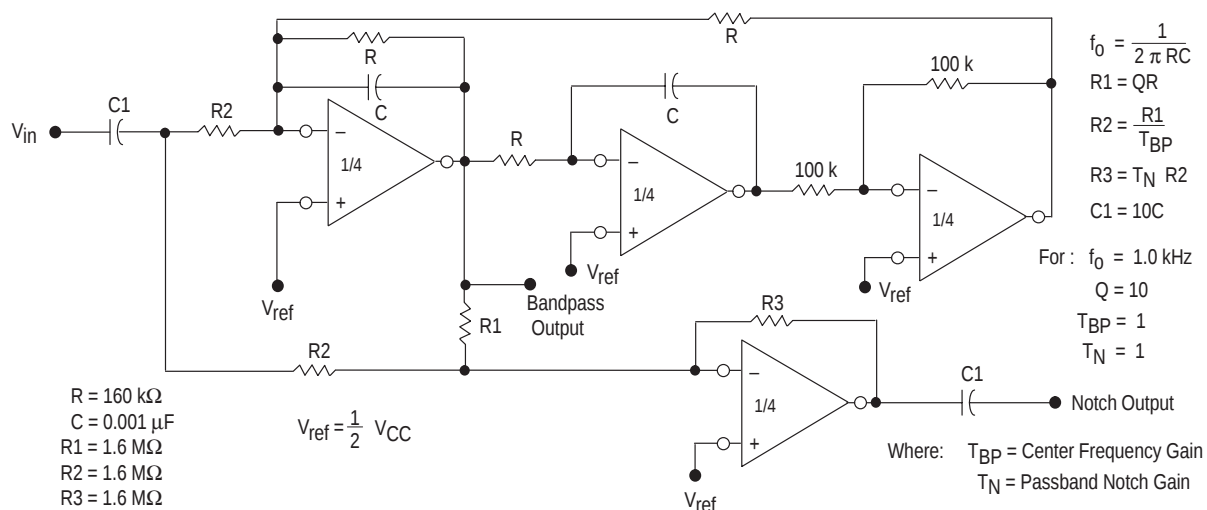
Figure 14. Bi-Quad Filter
