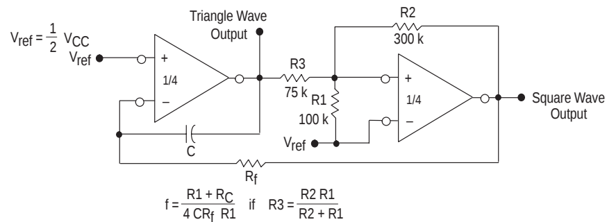
Figure 13. Function Generator
