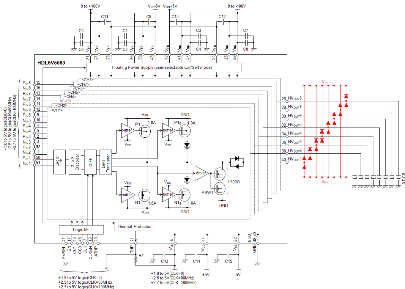
Fig. 2-(b) Typical Application Circuit-2
