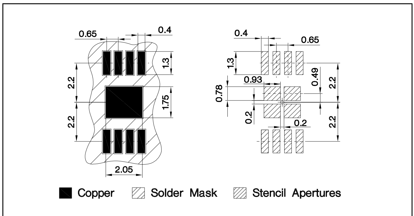
Figure 28 PG-TSSOP-8 footprint
