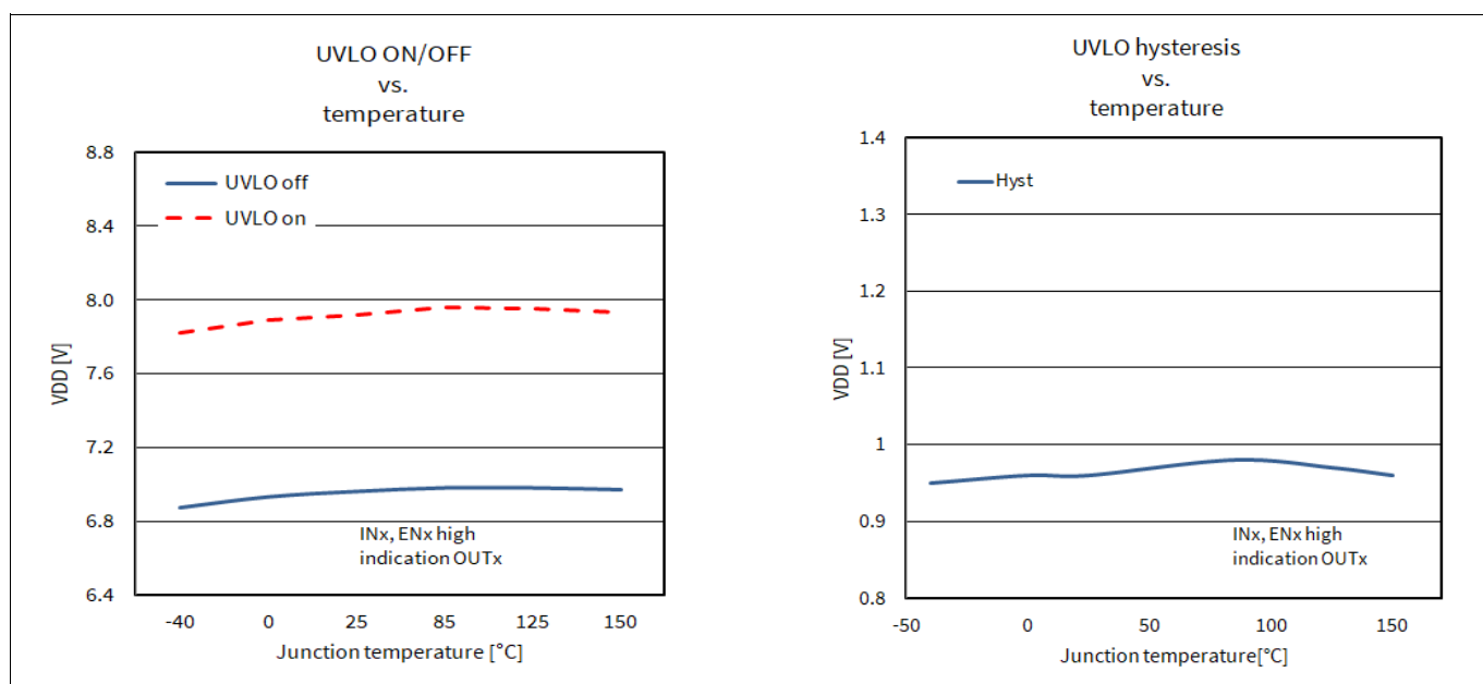
Figure 15 Typical undervoltage lockout behavior vs. temperature for 2EDN8x (8 V)
