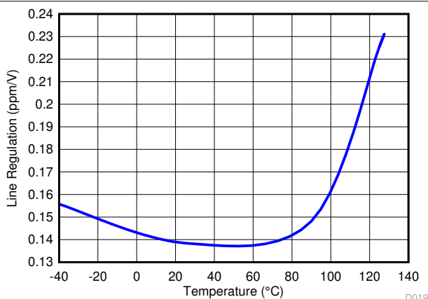
Figure 7-6. Line Regulation
