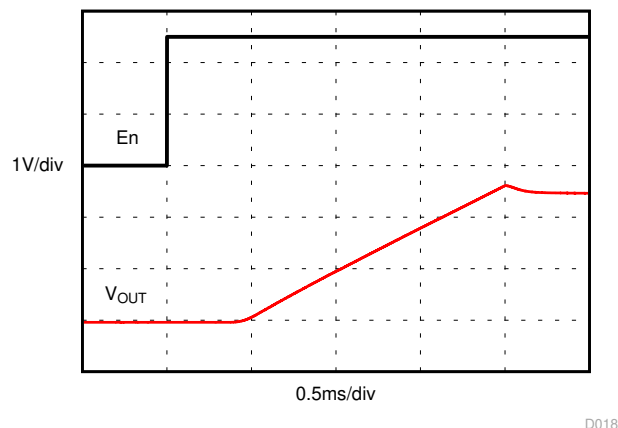
Figure 7-20. Turnon Time (Enable)
