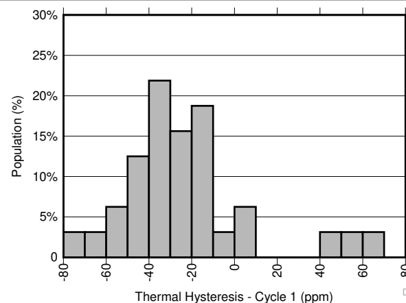
Figure 7-17. Thermal Hysteresis Distribution (Cycle 1)
