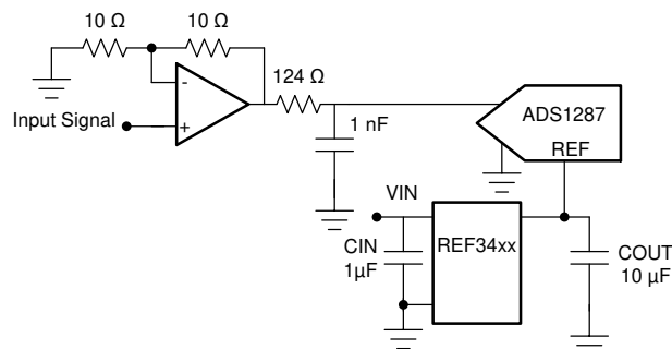
Simplified Schematic
