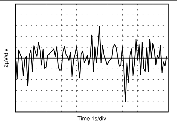
Figure 7-21. 0.1-Hz to 10-Hz Noise ( V_{OUT} )
