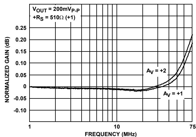
FIGURE 19. GAIN FLATNESS
