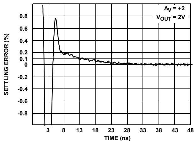
FIGURE 23. SETTLING RESPONSE
