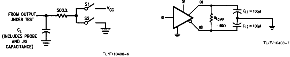
FIGURE 5. Driver Propagation Delay and Transition Time Test Circuits
