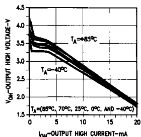
Receiver VOH vs IOH vs Temperature
