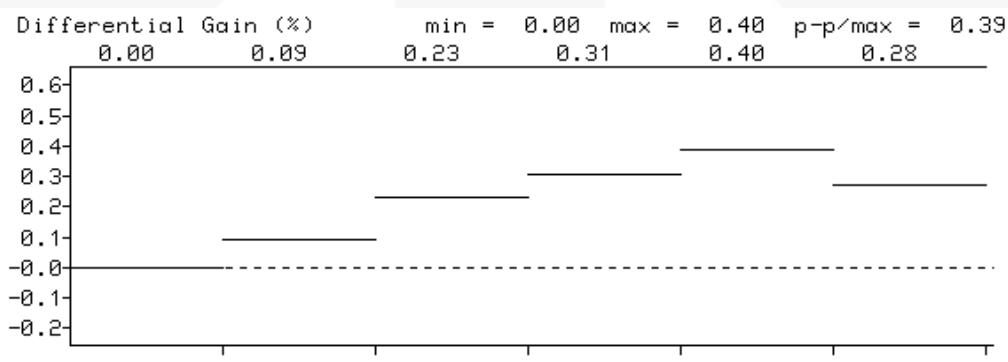
Figure 7. Differential Gain
