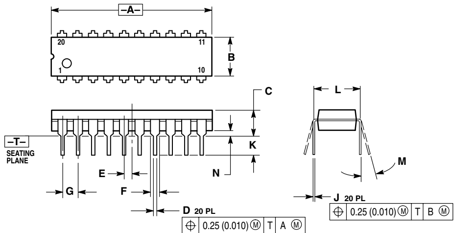
Figure 17-1. 20-Pin PDIP (Case #738)
