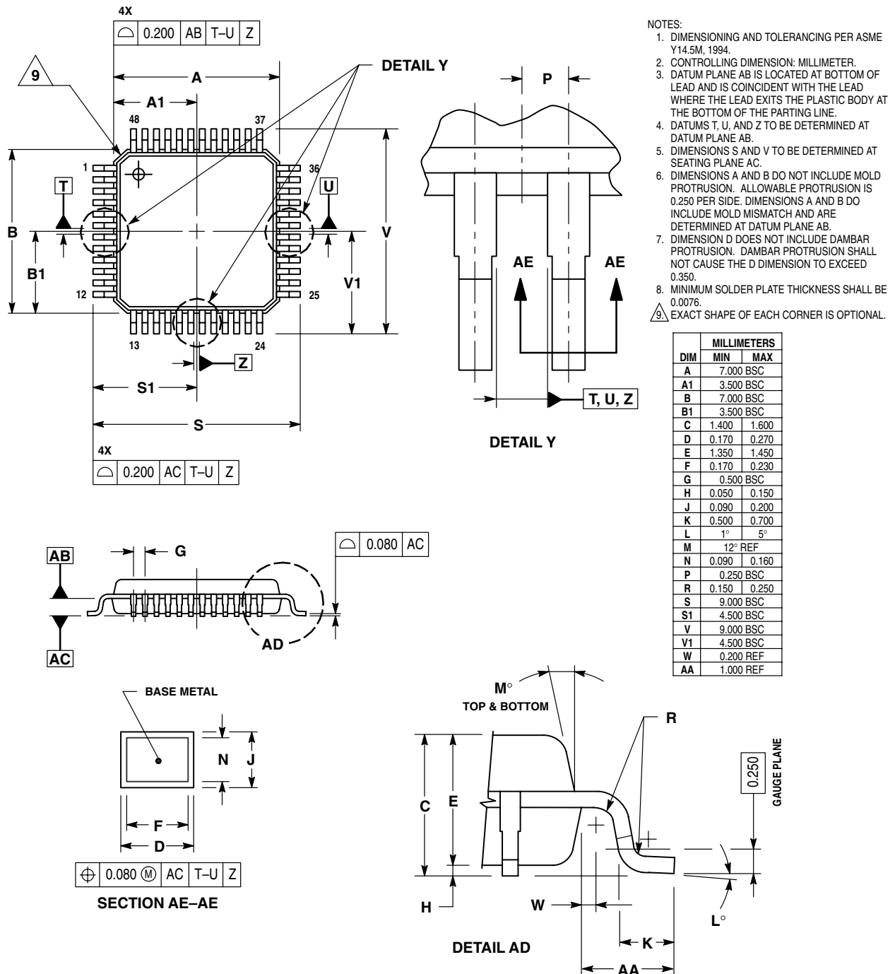
Figure 17-5. 48-Pin LQFP (Case #932)
