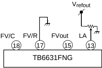
<Application circuit example>
