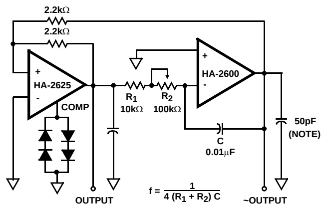
FIGURE 2. FUNCTION GENERATOR
