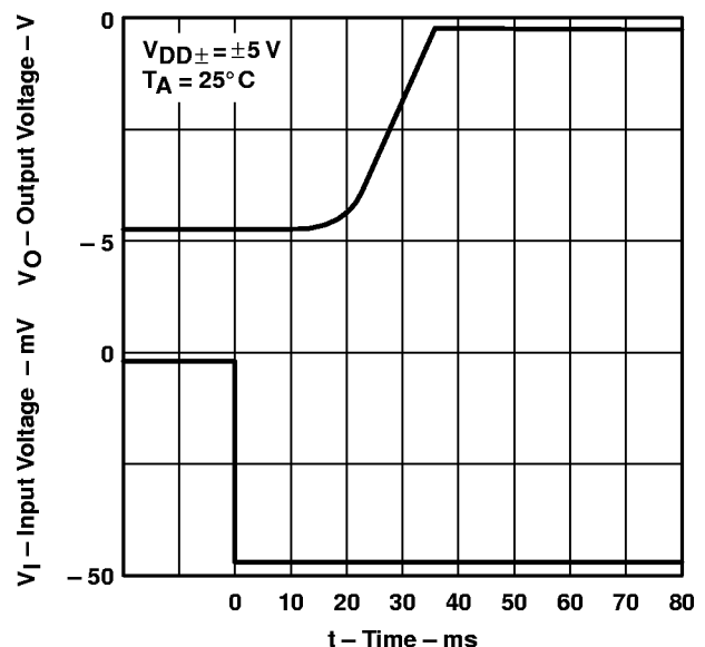
Figure 34. Overload Recovery
