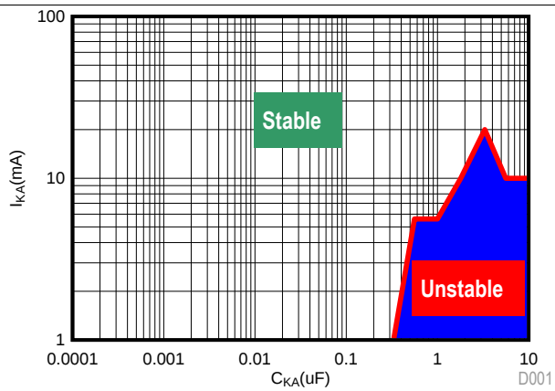
Figure 19. High I_{KA} ( V_{KA} = 5.0 V) Stability Boundary Conditions all ATL43xx Devices
