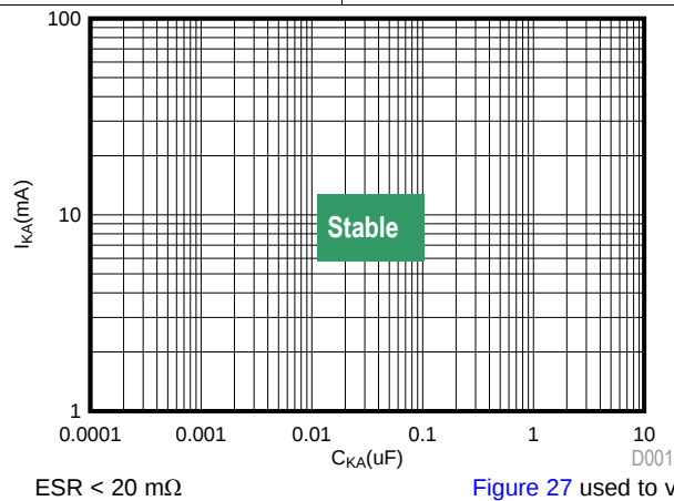
Figure 21. High I_{KA} ( V_{KA} = 15.0 V) Stability Boundary Conditions all ATL43xx Devices
