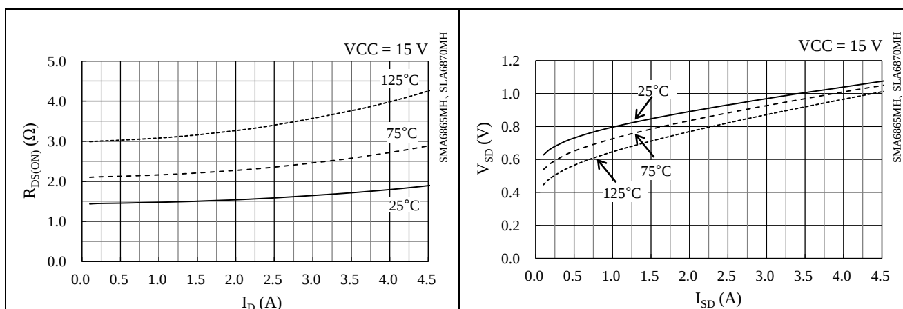
Figure 14-35. Power MOSFET R_{DS(ON)} vs. I_D
