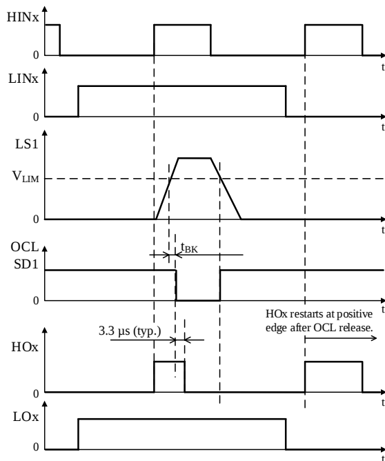
Figure 11-16. OCL Operational Waveforms (OCL = SD)
