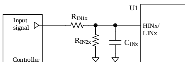
Figure 11-8. Filter Circuit for HINx or LINx Pin
