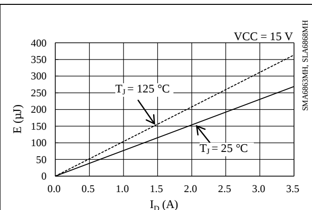
Figure 14-42. Low-side Switching Loss
