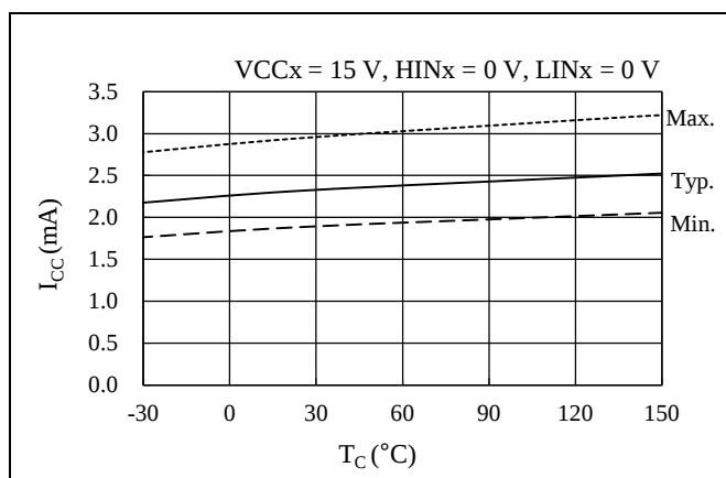
Figure 14-3. Logic Supply Current, I_{CC} vs. T_C ( HIN_x = 0 V, LIN_x = 0 V)
