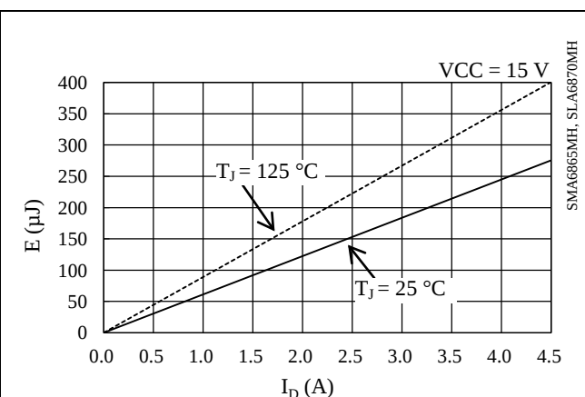
Figure 14-44. Low-side Switching Loss
