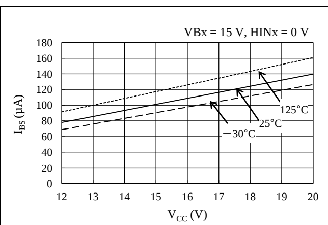
Figure 14-8. V_B Pin Voltage, V_B vs. Logic Supply Current, I_{BS} ( HIN_x = 0 V)
