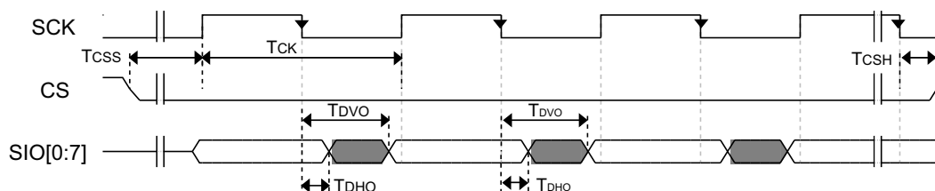
Figure 40. FlexSPI output timing in SDR mode
