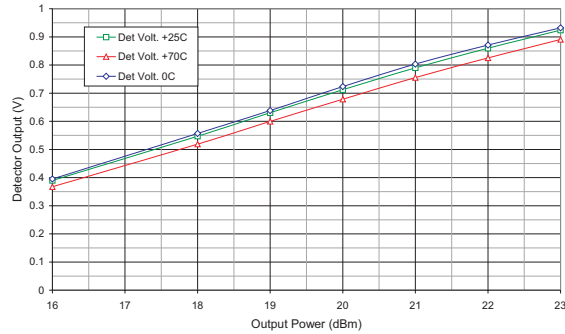
Figure 11: Power Detector Voltage vs. Output Power at 2.437 GHz, 3.3 V (IEEE 802.11b @ 11 Mbps)
