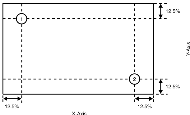
FIGURE 5. Two Points Calibration Mapping
