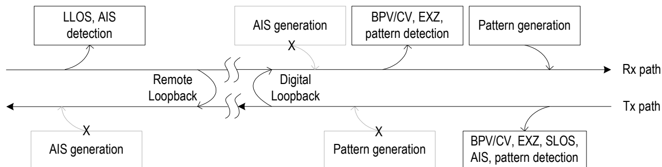
Figure-36 Priority Of Diagnostic Facilities During Manual Remote Loopback + Automatic Digital Loopback
