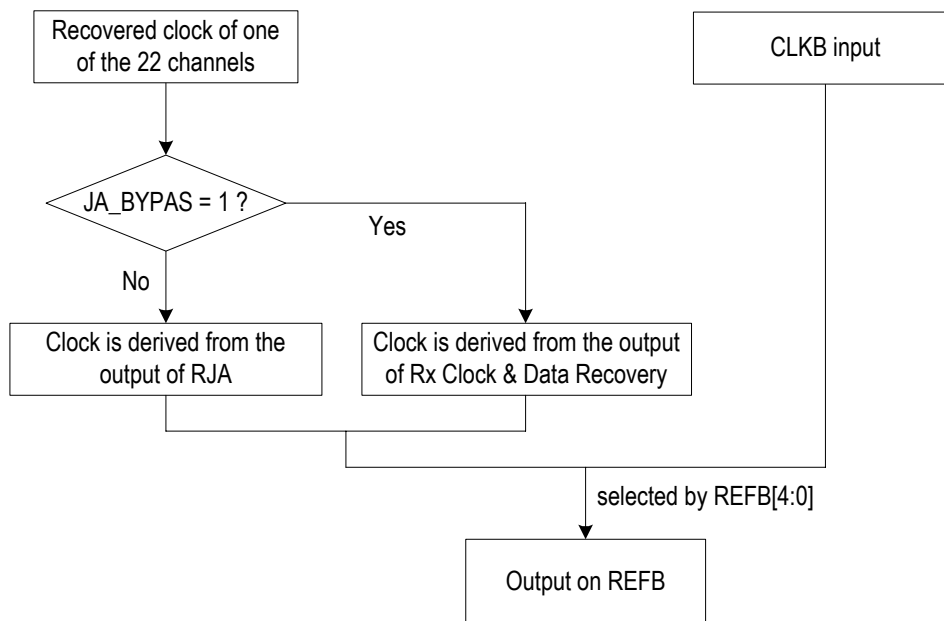
Figure-41 REFB Output Options in Normal Operation
