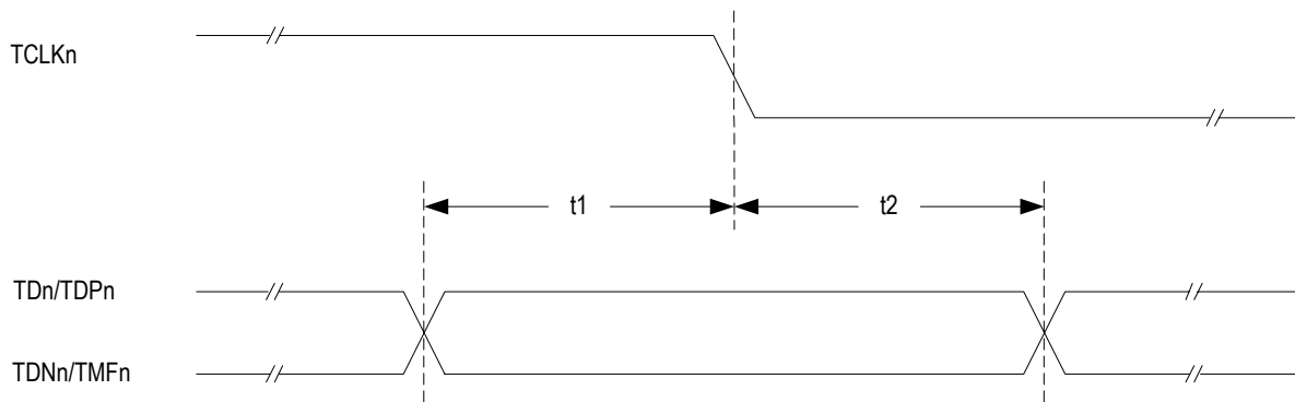
Figure-51 Transmit Clock Timing Diagram
