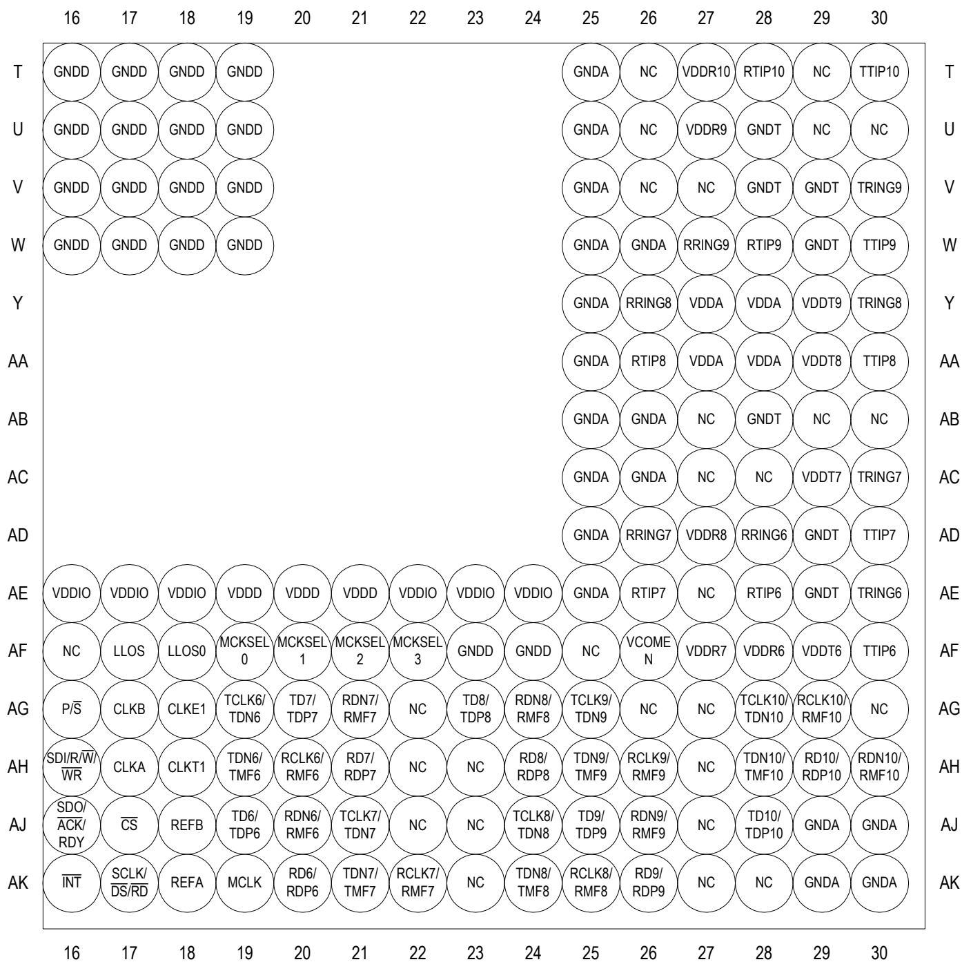
Figure-6 640-Pin TEPBGA (Top View) - Bottom Right
