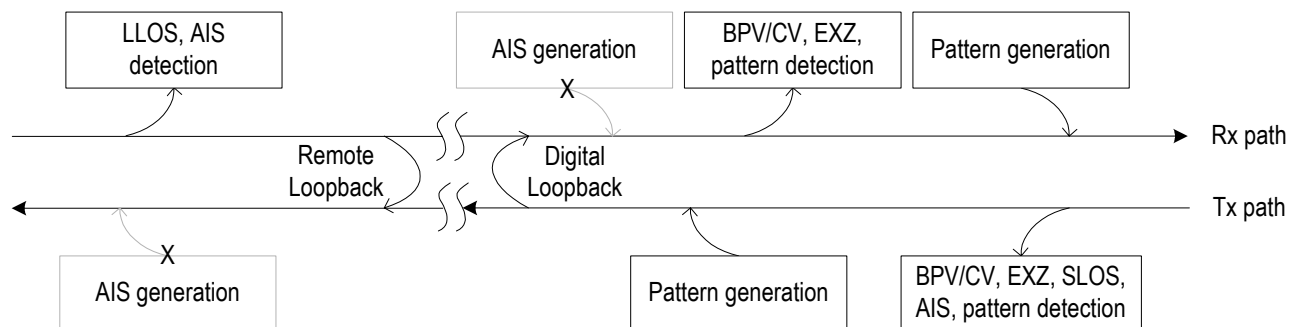
Figure-35 Priority Of Diagnostic Facilities During Manual Remote Loopback + Manual Digital Loopback
