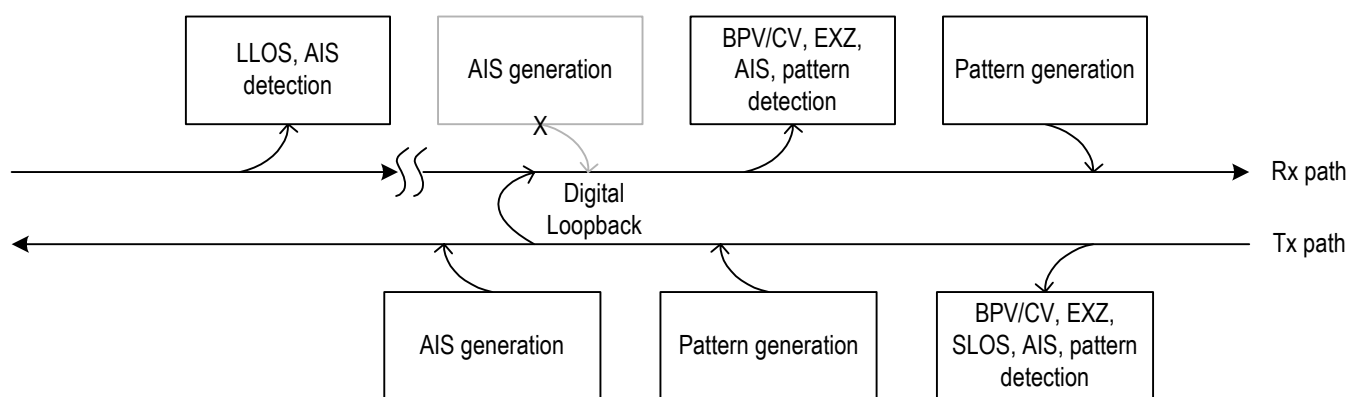
Figure-34 Priority Of Diagnostic Facilities During Digital Loopback
