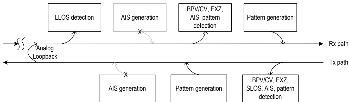
Figure-32 Priority Of Diagnostic Facilities During Analog Loopback
