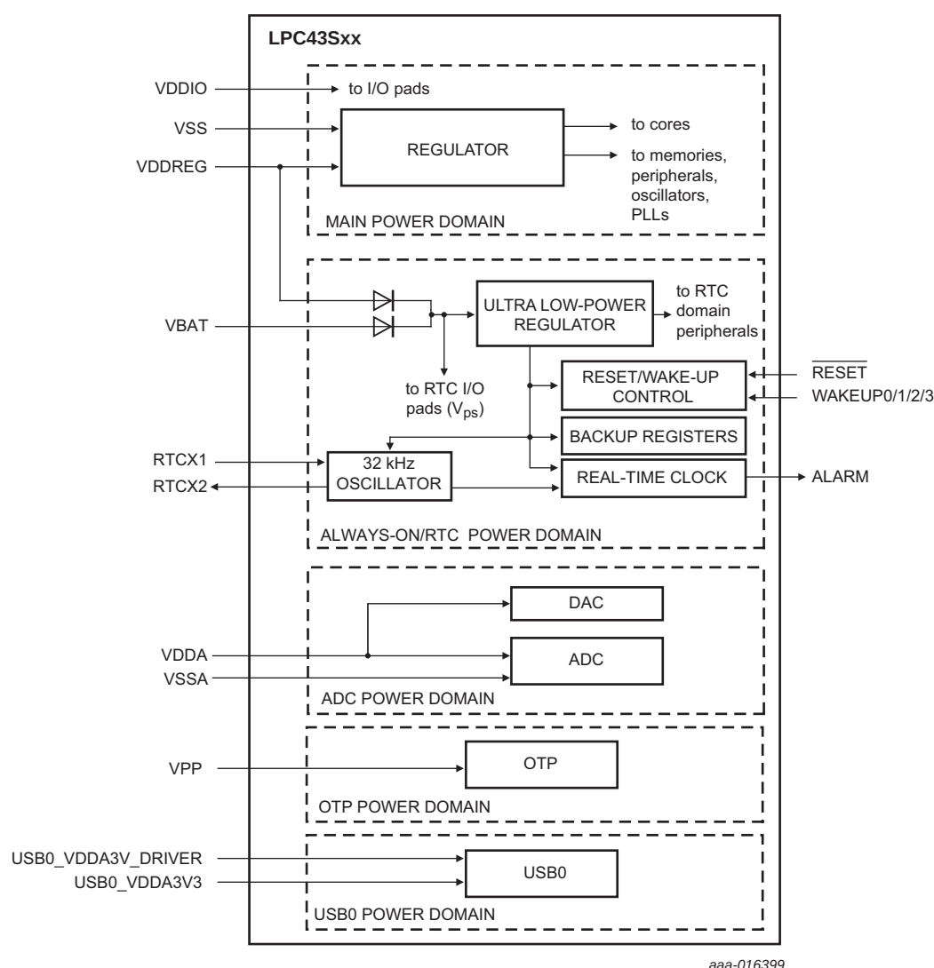
Fig 7. Power domains
