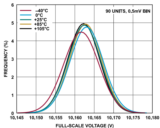
Figure 48. Full-Scale Voltage Distribution, 0 V to 10 V Range
