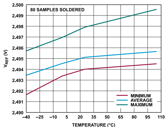
Figure 69. V_{REF} vs. Temperature
