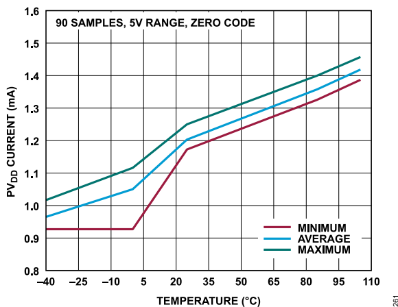
Figure 76. PV_{DD} Current vs. Temperature
