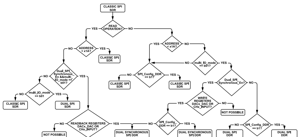
Figure 98. Register Access Modes
