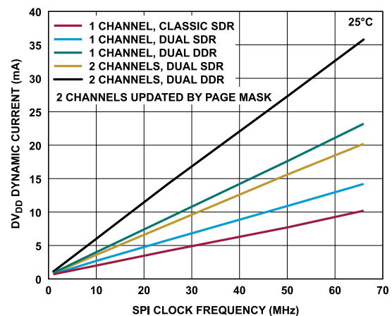
Figure 70. AD3542R-16 DV_{DD} Dynamic Current vs. SPI Clock Frequency, SPI Mode
