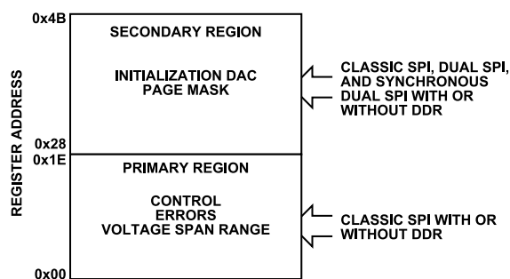
Figure 95. Register Access Modes
