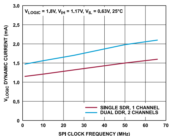
Figure 72. V_{LOGIC} Dynamic Current vs. SPI Clock Frequency, SPI Mode
