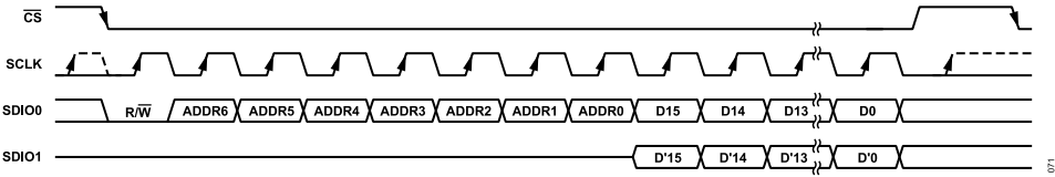
Figure 94. Synchronous Dual SPI Mode
