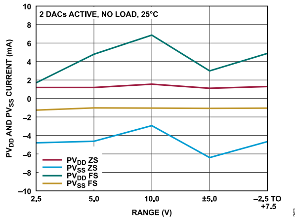
Figure 78. PV_{DD} and PV_{SS} Current vs. Range
