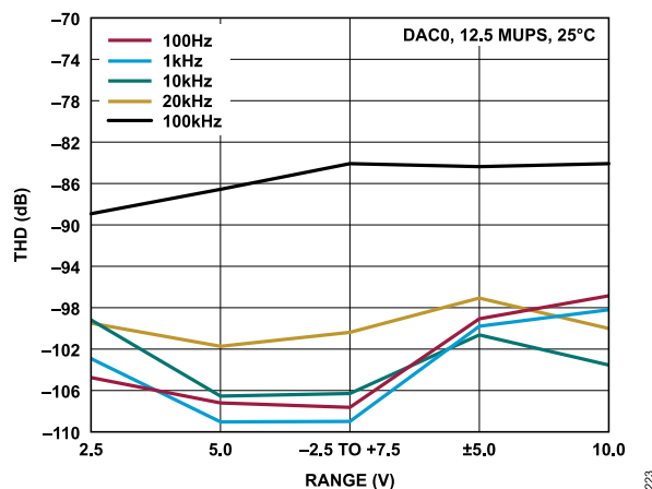
Figure 36. AD3542R-16 THD vs. Range
