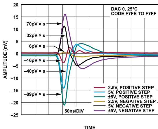
Figure 53. Digital-to-Analog Glitch
