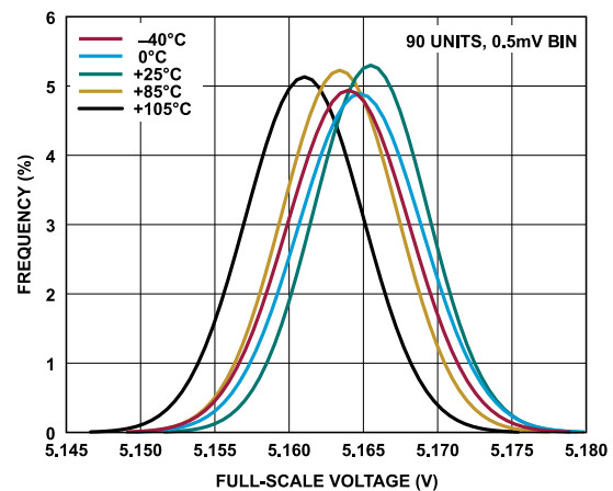
Figure 49. Full-Scale Voltage Distribution, -5 V to +5 V Range
