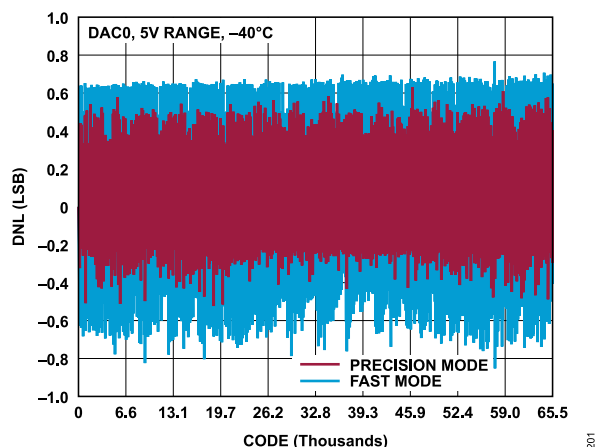
Figure 11. AD3542R-16 DNL vs. Code, 0 V to 5 V Range, -40^\circ\text{C} , Fast Mode and Precision Mode
