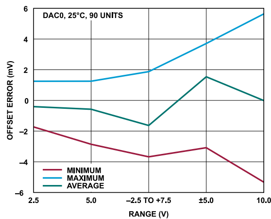
Figure 27. Offset Error vs. Range
