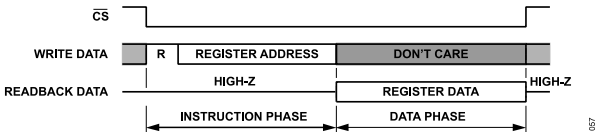
Figure 81. Basic SPI Read Frame
