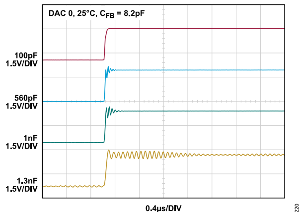
Figure 32. Output Load Stability ( C_{FB} Is Feedback Capacitor)
