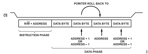
Figure 87. Looping Enabled with STREAM_MODE = 2
