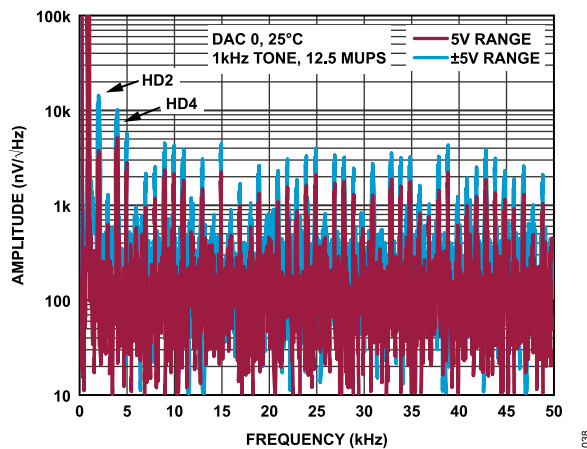
Figure 38. AD3542R-12 Spectral Noise Density with 1 kHz Sine Wave Playback
