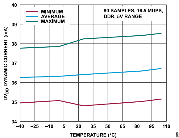
Figure 74. AD3542R-16 DV_{DD} Dynamic Current vs. Temperature
