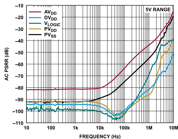
Figure 64. AC PSRR vs. Frequency
