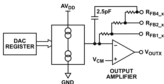
Figure 79. DAC Channel Architecture Block Diagram
