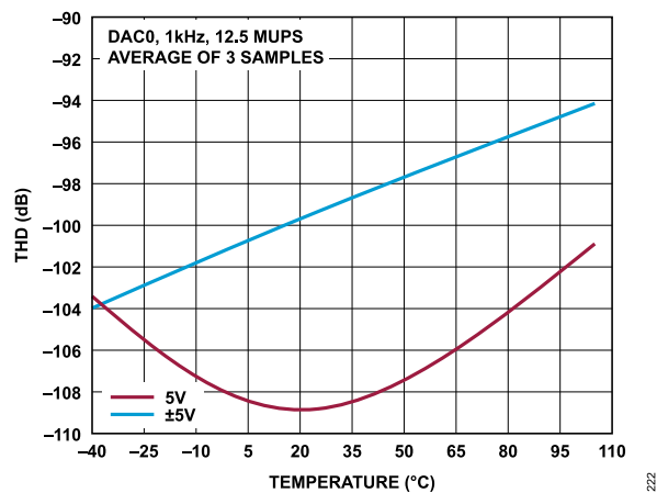
Figure 35. AD3542R-16 THD vs. Temperature
