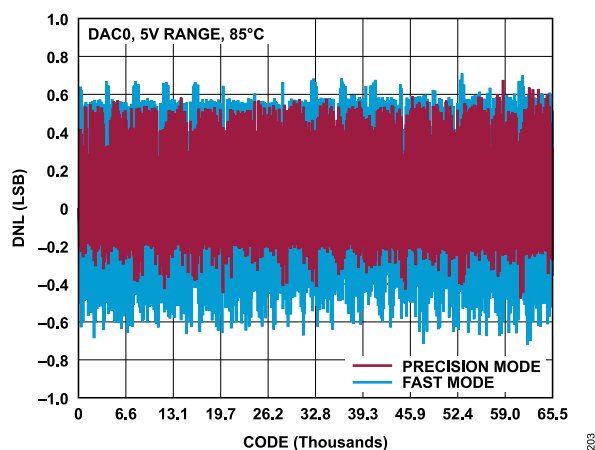
Figure 13. AD3542R-16 DNL vs. Code, 0 V to 5 V Range, 85^\circ\text{C} , Fast Mode and Precision Mode
