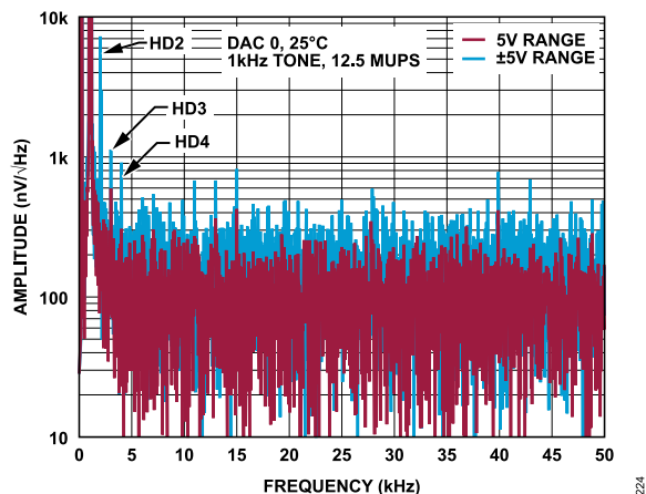
Figure 37. AD3542R-16 Spectral Noise Density with 1 kHz Sine Wave Playback
