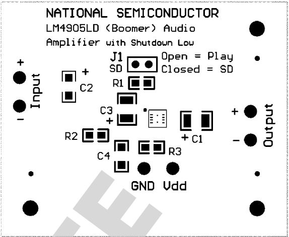
Silk Screen
