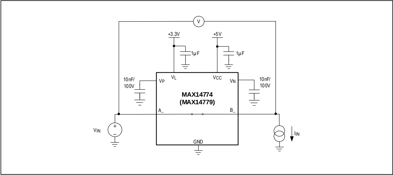
Figure 1. On-Resistance Measurement
