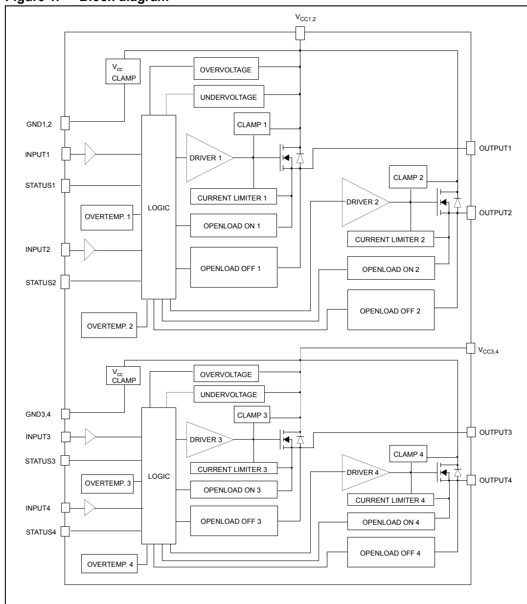
Figure 1. Block diagram
