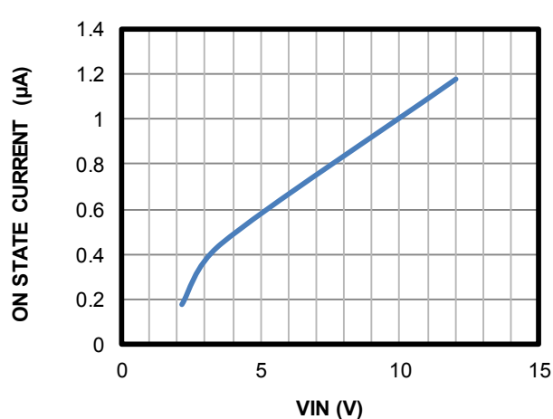
On-State Current vs. V_{IN}
