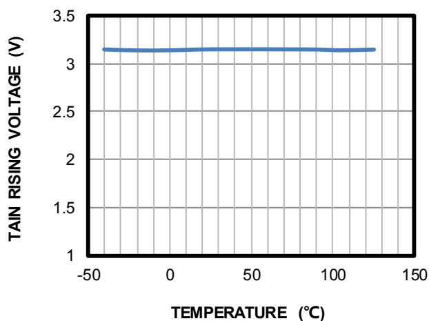
TAIN Rising Voltage vs. Temperature
