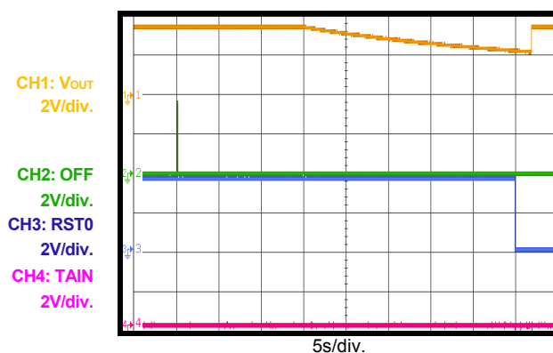
Shipping Mode Exit with RST0
