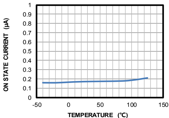
On-State Current vs. Temperature
