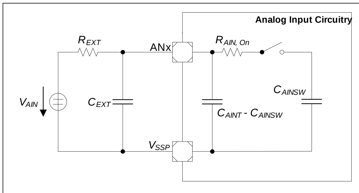
Figure 10 ADC Input Circuits
