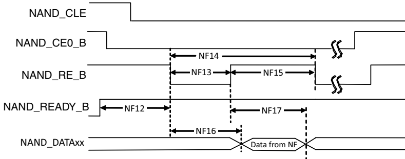
Figure 27. Read Data Latch Cycle Timing Diagram (EDO Mode)
