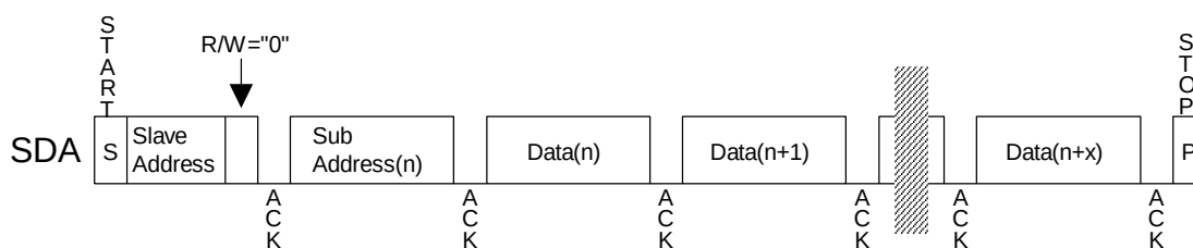
Figure 24. Data Transfer Sequence at the I 2 C-Bus
