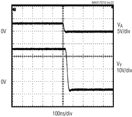
SCAN DRIVER PROPAGATION DELAY (FALLING EDGE)
