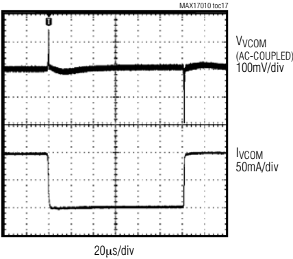
OPERATIONAL AMPLIFIER LOAD-TRANSIENT RESPONSE
