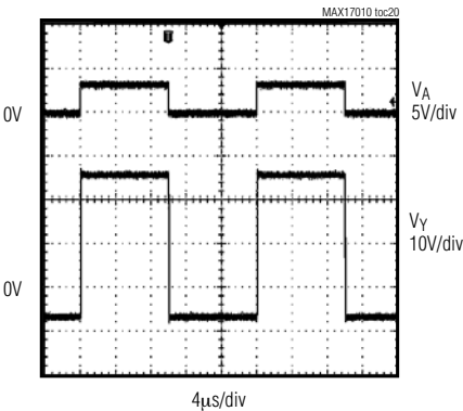
SCAN DRIVER INPUT/OUTPUT WAVEFORMS WITH LOGIC INPUT
