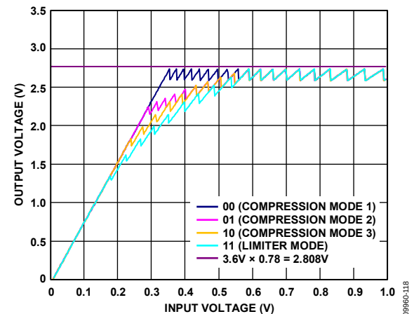
Figure 32. Adjustable Compression Settings, PVDD = 3.6 V, ALC Threshold Level = 78%
