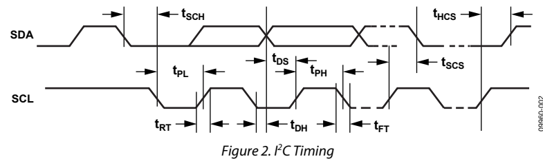
Figure 2. I 2 C Timing
