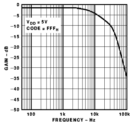
Figure 18. AD7395 Reference Multiplying Bandwidth
