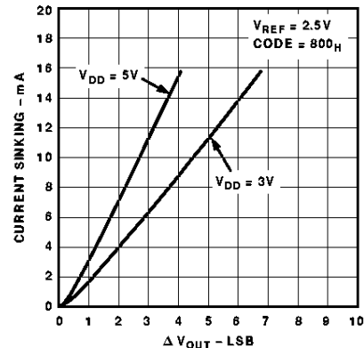
Figure 15. AD7394 I_{OUT} Sink Current vs. \Delta V_{OUT}
