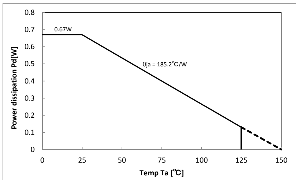
Figure 21. Power Dissipation
