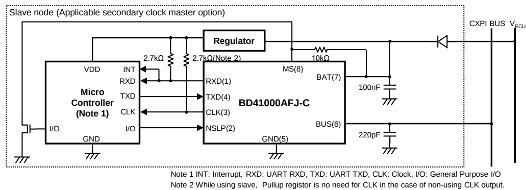
Figure 20. Application Example of Secondary Clock Master Option
