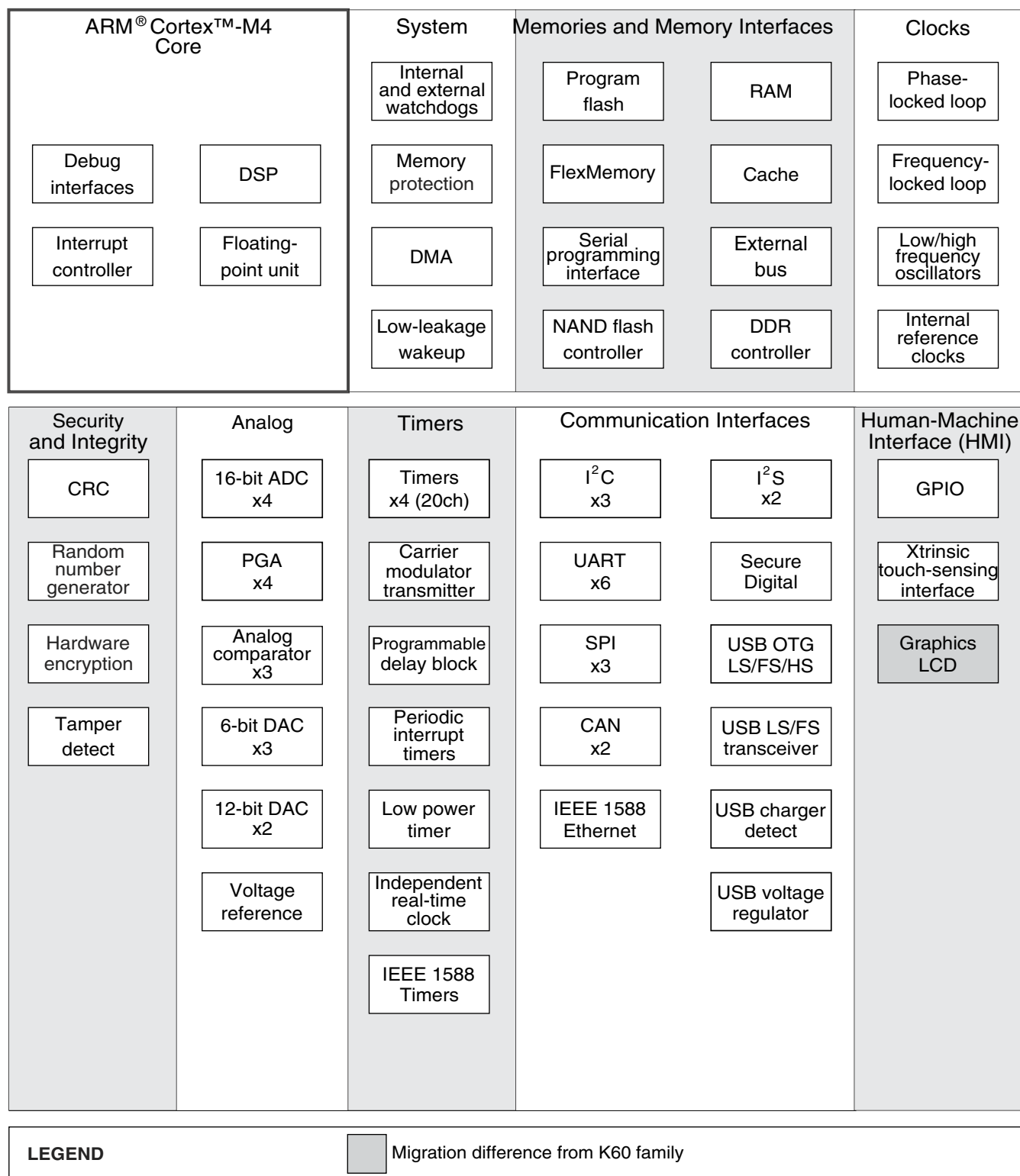
Figure 2. K70 Block Diagram
