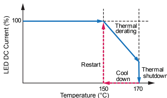
Figure 9: Thermal Derating and Shutdown Protection Features
