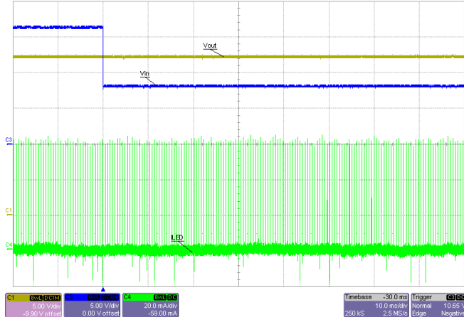
Transient Response to Step-Change In V_{IN} (16V to 8V) PWM Duty Cycle 0.02%
