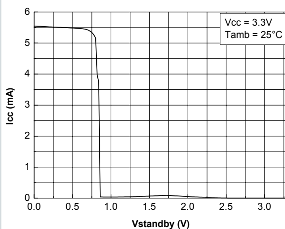
Figure 77. Current consumption vs standby voltage @ V_{cc} = 3.3\text{ V}
