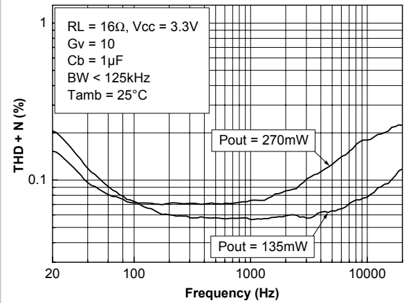
Figure 67. THD + N vs frequency, R_L=16\ \Omega , G_v=10 , V_{CC}=3.3\text{ V}
