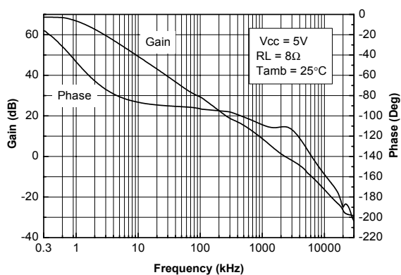
Figure 2. Open loop frequency response V_{CC}=5\text{ V}
