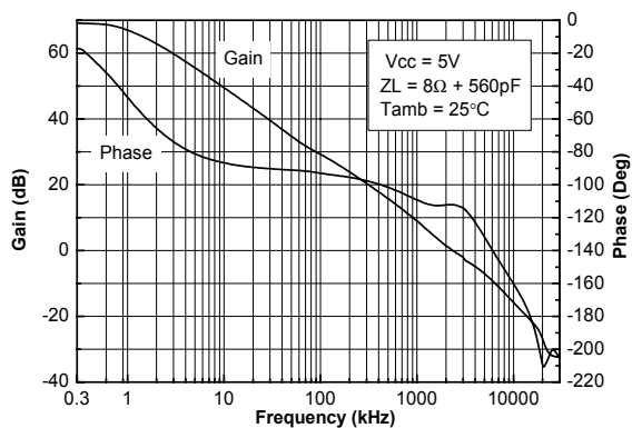
Figure 3. Open loop frequency response Z_L=8\ \Omega
