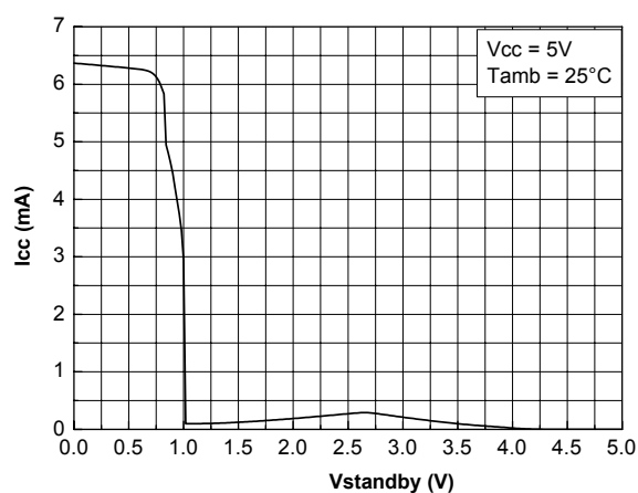
Figure 75. Current consumption vs standby voltage @ V_{cc} = 5\text{ V}
