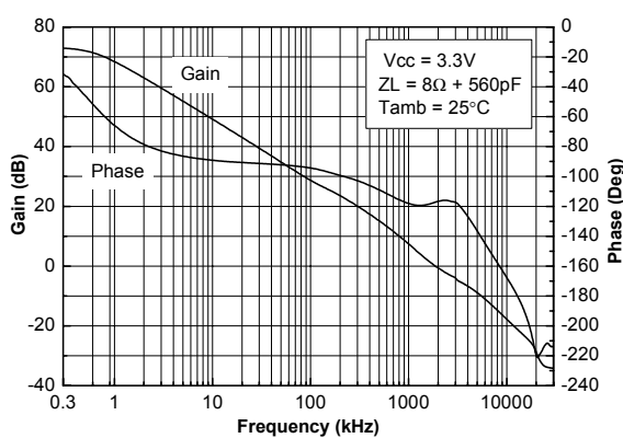
Figure 5. Open loop frequency response V_{CC}=3.3\text{ V} , Z_L=8\ \Omega
