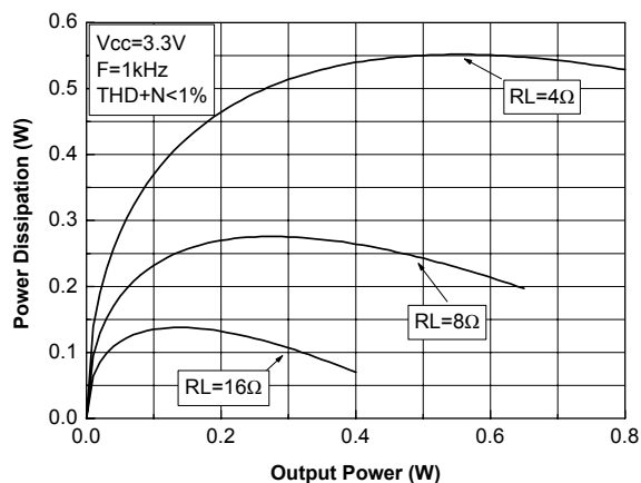
Figure 19. Power dissipation vs Pout Vcc=3.3 V
