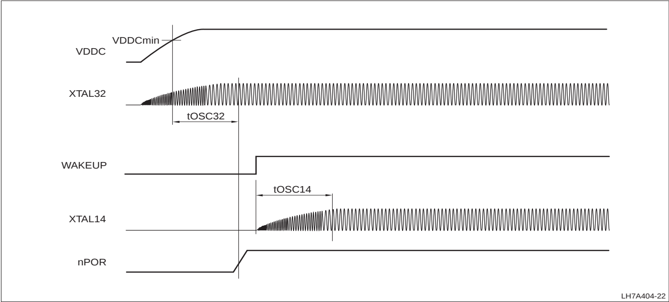
Figure 48. PLL Start-up
