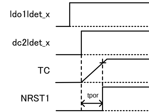
Fig.7.3 Power-on reset
