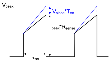
Typical Waveform
