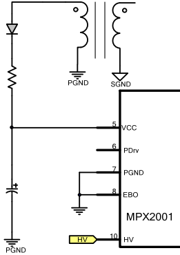
Figure 11: Start-Up Circuit
