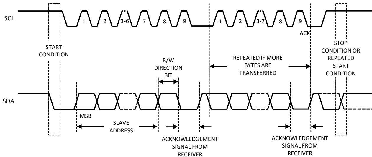
Figure 4. Data Transfer on I²C Serial Bus
