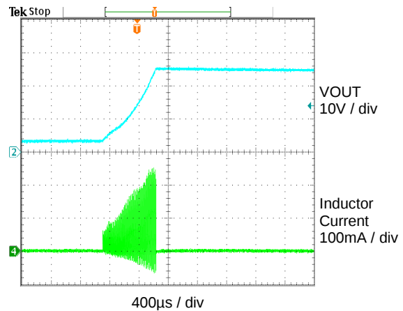
Turn On with LED Open (OVP = 25.9V)
