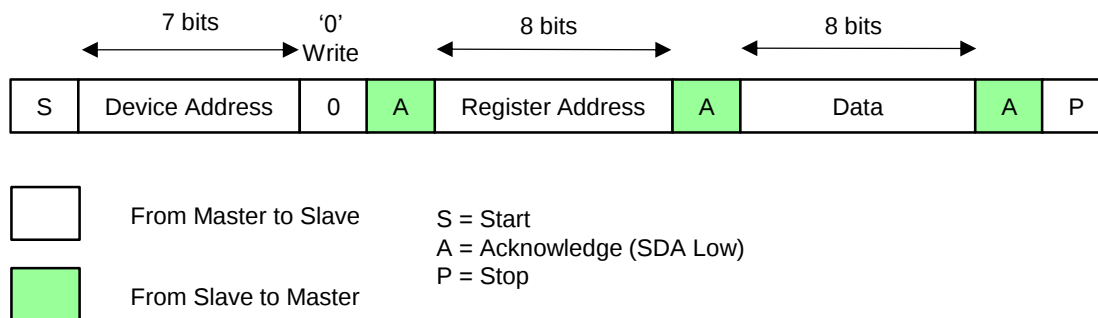
Figure 5. I²C Write Cycle
