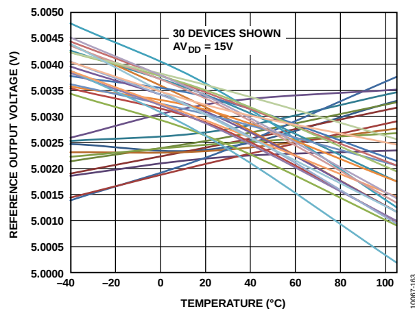
Figure 41. REFOUT Voltage vs. Temperature (When the AD5737 is soldered onto a PCB, the reference shifts due to thermal shock on the package. The average output voltage shift is -4 mV. Measurement of these parts after seven days shows that the outputs typically shift back 2 mV toward their initial values. This second shift is due to the relaxation of stress incurred during soldering.)
