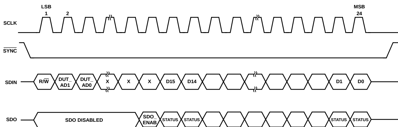
Figure 6. Status Readback During a Write
