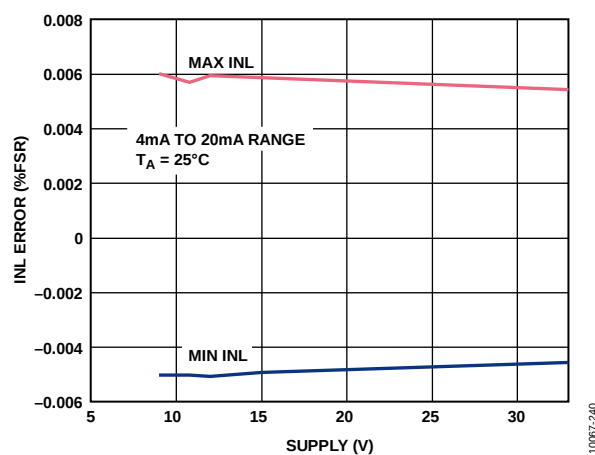
Figure 18. Integral Nonlinearity Error vs. Supply, External R_{SET}
