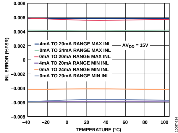
Figure 12. Integral Nonlinearity Error vs. Temperature, Internal R_{SET}
