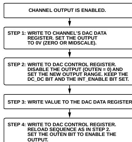
Figure 52. Programming Sequence to Change the Output Range
