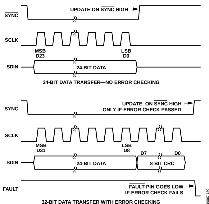
Figure 54. PEC Timing
