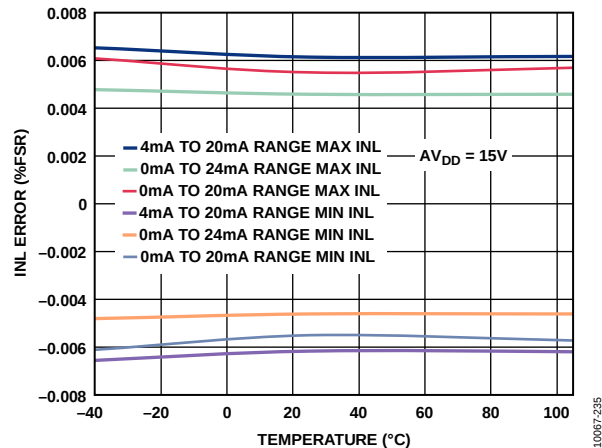
Figure 13. Integral Nonlinearity Error vs. Temperature, External R_{SET}
