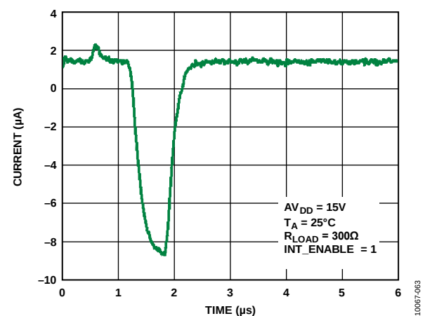
Figure 25. Current vs. Time on Output Enable
