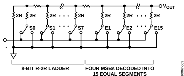
Figure 48. DAC Ladder Structure
