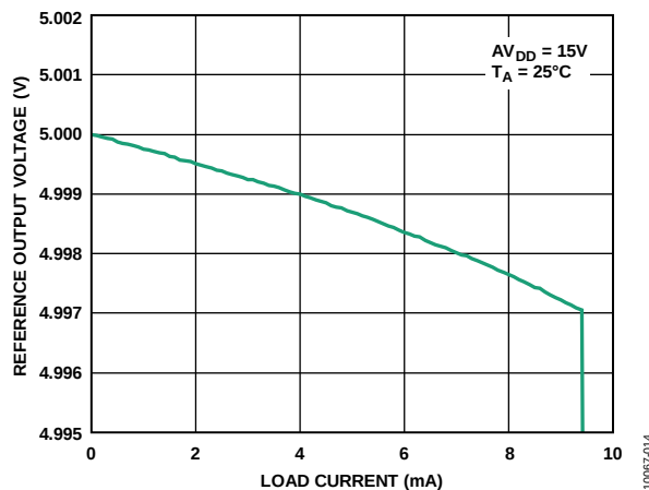
Figure 42. REFOUT Voltage vs. Load Current
