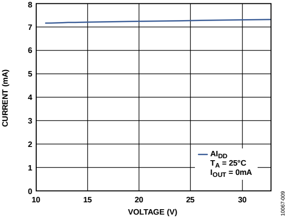
Figure 45. Supply Current ( A_{I_{DD}} ) vs. Supply Voltage ( A_{V_{DD}} )
