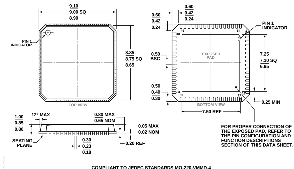
Figure 67. 64-Lead Lead Frame Chip Scale Package [LFCSP_VQ] 9 mm × 9 mm Body, Very Thin Quad (CP-64-3) Dimensions shown in millimeters
