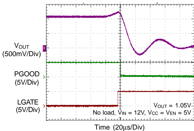
Over-Voltage Protection
