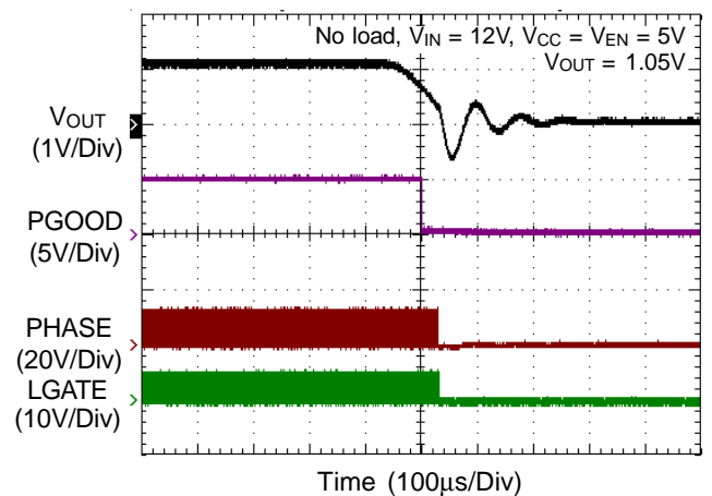
Under-Voltage Protection
